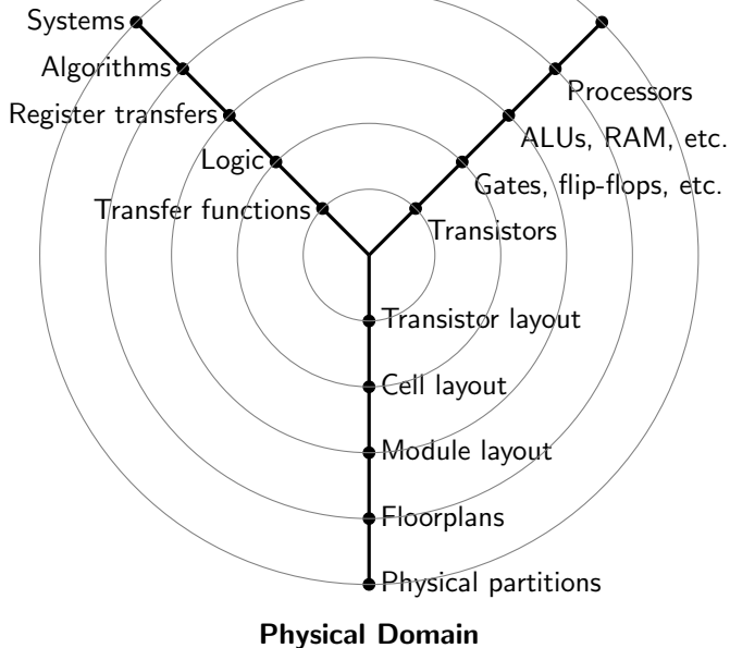
Figure 1: Gajski-Kuhn Y-chart
