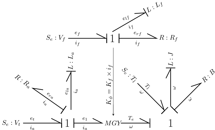
Figure 1: Bond graph model of a DC motor
