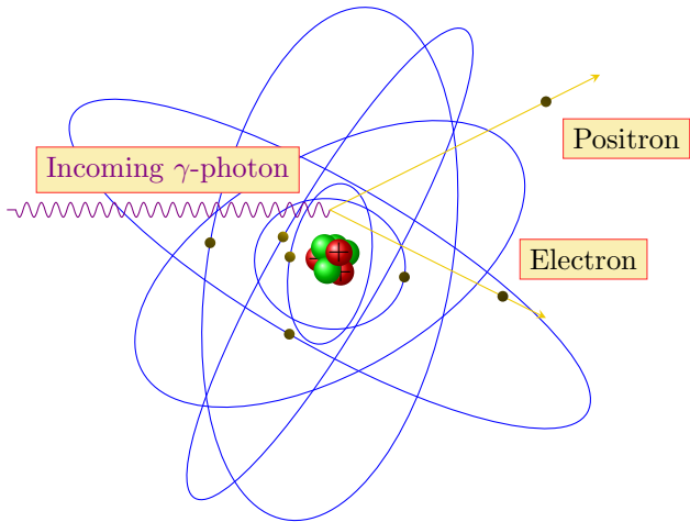
Figure 3: Pair creation.
