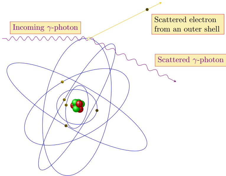
Figure 2: Compton scattering
